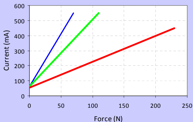
Current Curves
